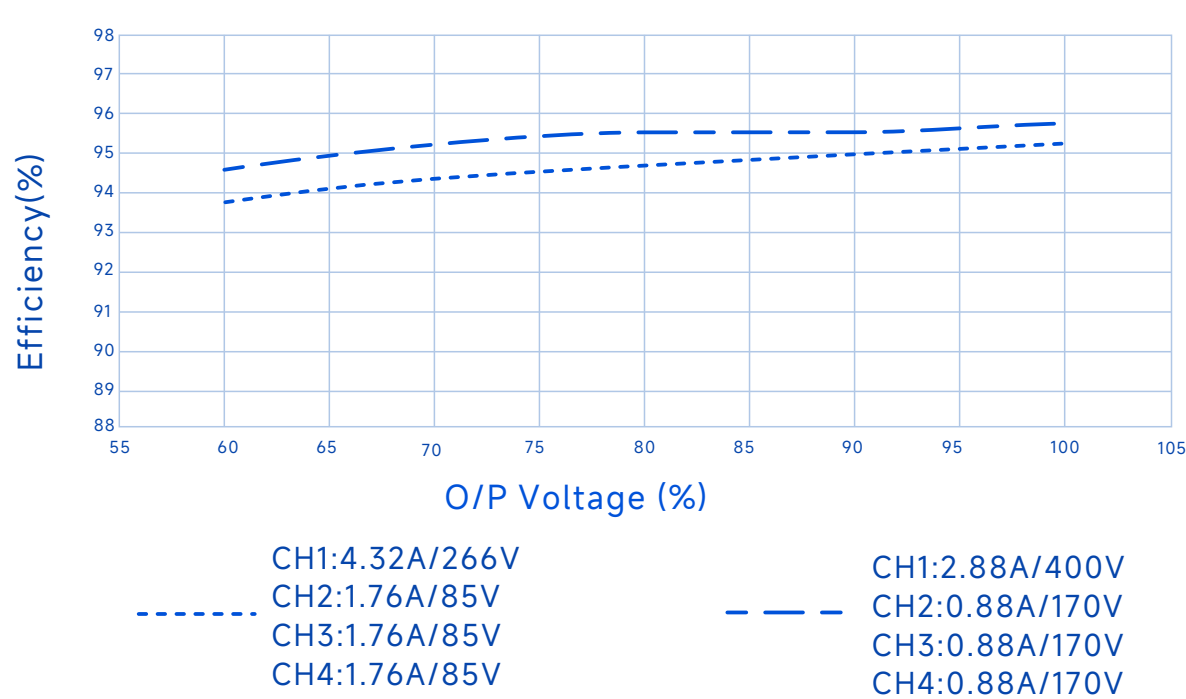
Efficiency Vs. O/P Voltage(Vin=347Vac)
