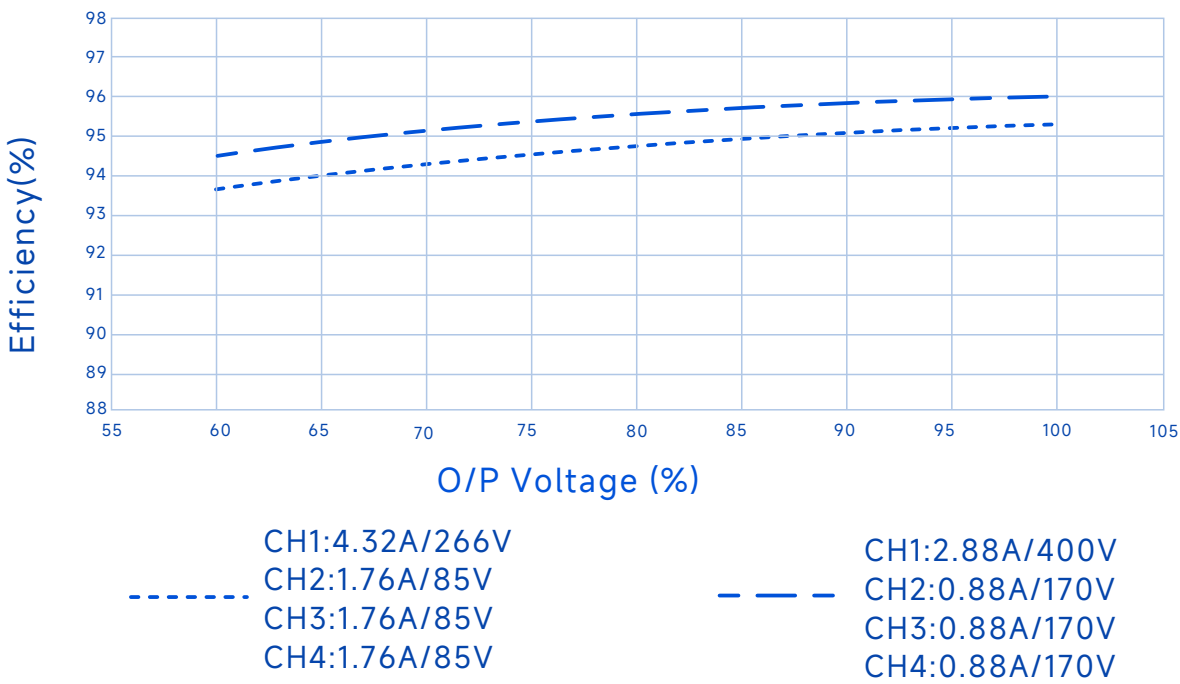
Efficiency Vs. O/P Voltage(Vin=480Vac)
